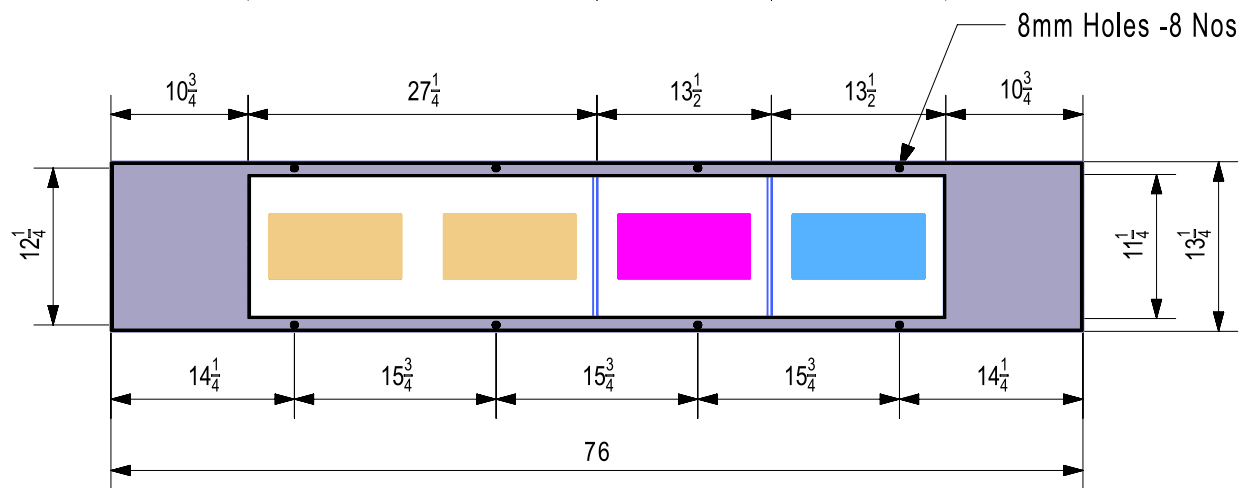
Machine Hopper Top View
