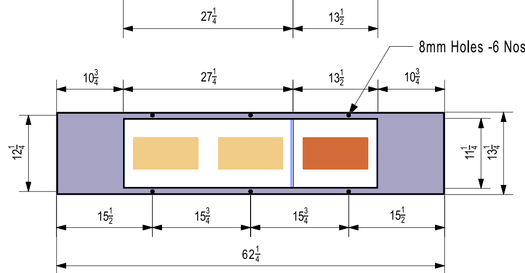
Machine Hopper Top View
